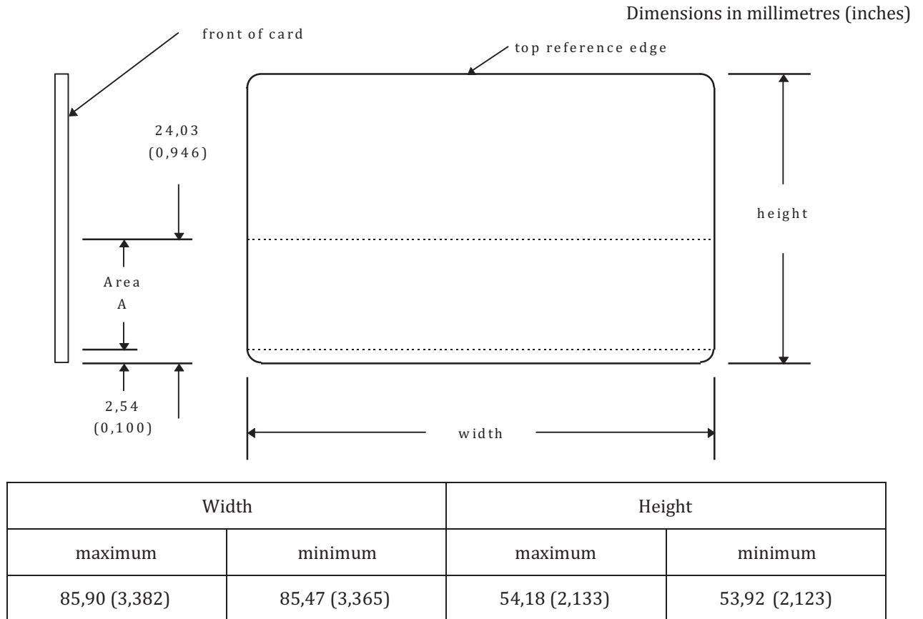
Figure 1 — Embossed card dimensions
