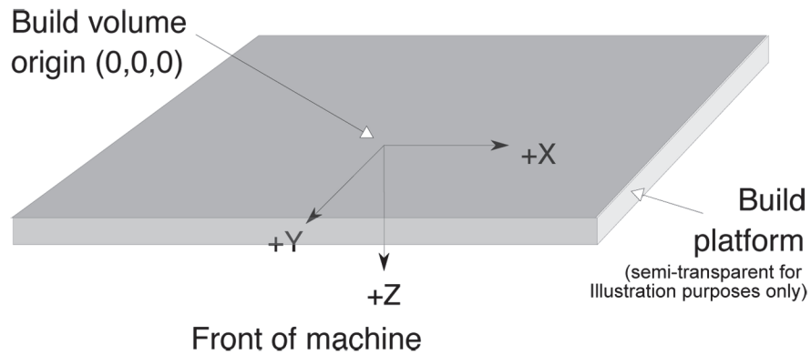
FIG. A1.2 Generic (Downward Building) Additive Manufacturing Machine/System
