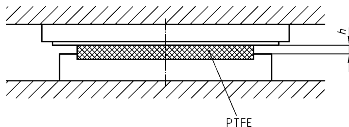
Figure 1 —Sliding part of combined bearings
