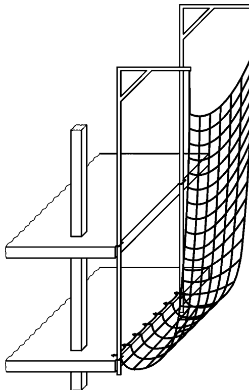
Figure 4 — Safety net System V (net with border rope attached to a gallow type support)
