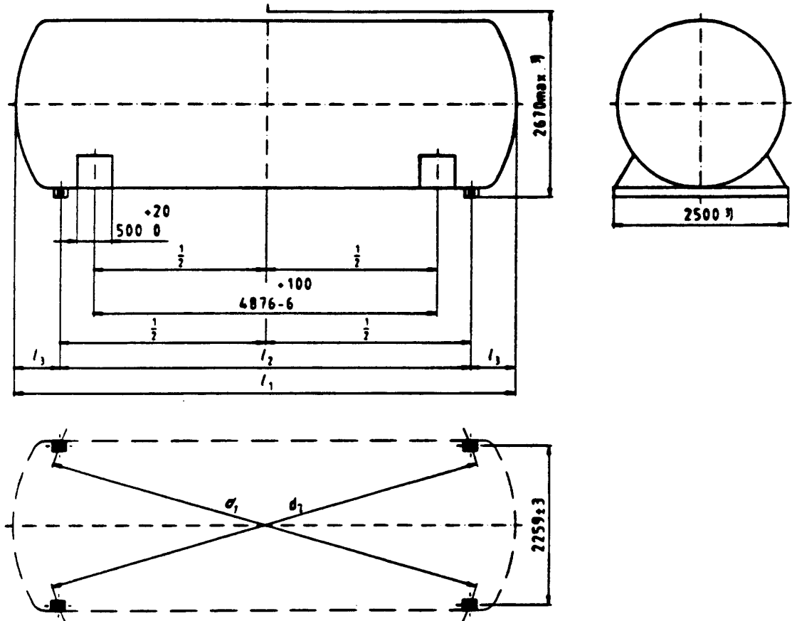
Figure 1: Dimensions for swap tanks
