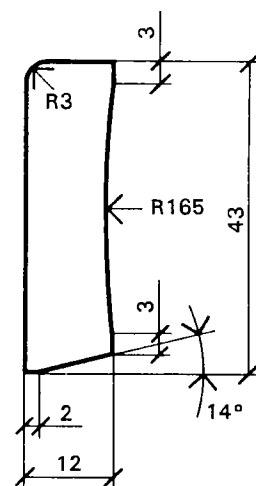
Sockellist 12x43
