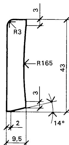
Sockellist 9,5x43
