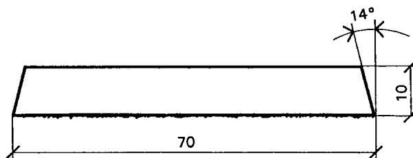
Gjutlist 10x70
