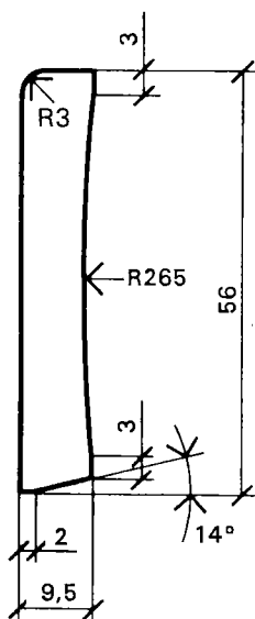
Sockellist 9,5x56
