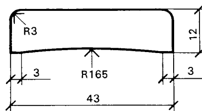
Foderlist 12x43
