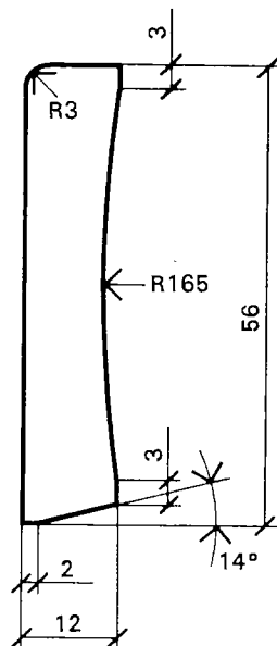
Sockellist 12x56
