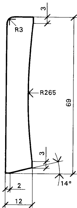
Sockellist 12x69
