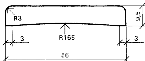
Foderlist 9,5x56
