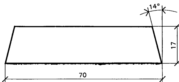
Gjutlist 17x70
