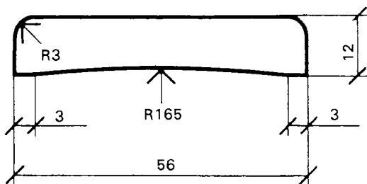
Foderlist 12x56
