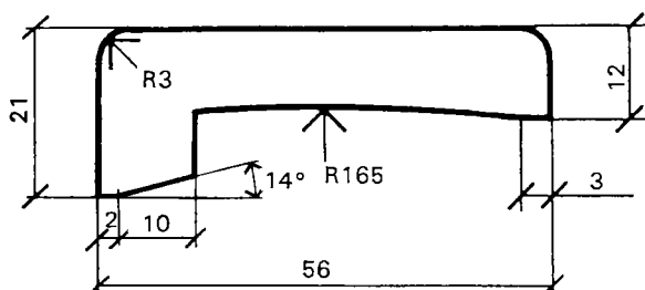
Klackfoder 21x56
