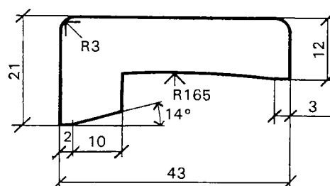
Klackfoder 21x43
