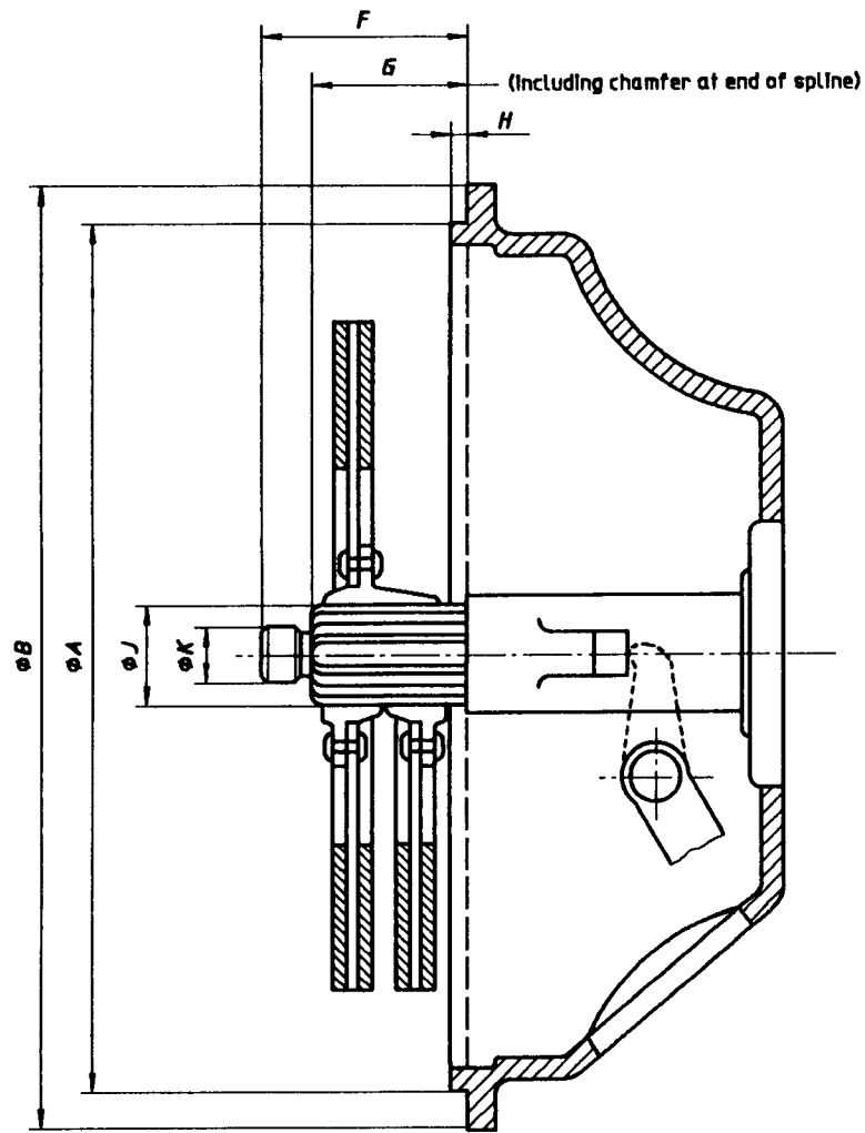
Figure 1 — Clutch housing
