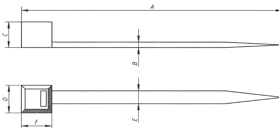
Figure 1 — Cable tie
